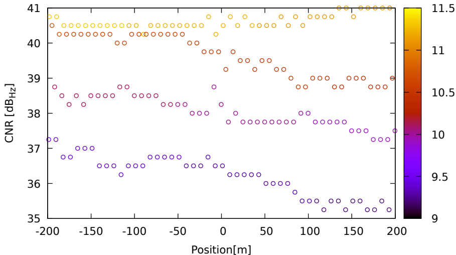
CNR vs position for E33 (E5a) on Xiaomi11T - DOY 263 jam. 2
