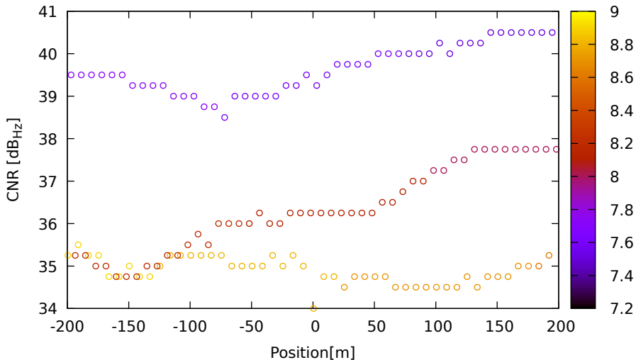
CNR vs position for E33 (E5a) on Xiaomi11T - DOY 263 jam. 3
