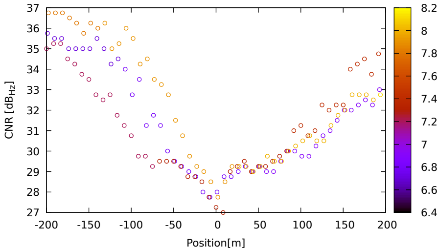
CNR vs position for E36 (E5a) on Xiaomi11T - DOY 263 jam. 1
