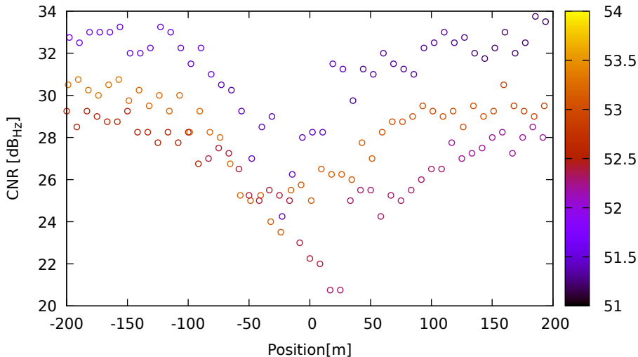
CNR vs position for G01 (L5) on Xiaomi11T - DOY 263 jam. 1
