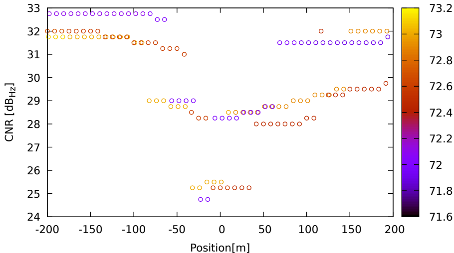
CNR vs position for G03 (L5) on Xiaomi11T - DOY 263 jam. 1
