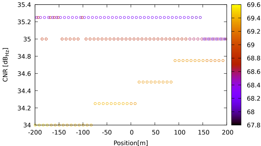
CNR vs position for G03 (L5) on Xiaomi11T - DOY 263 jam. 3
