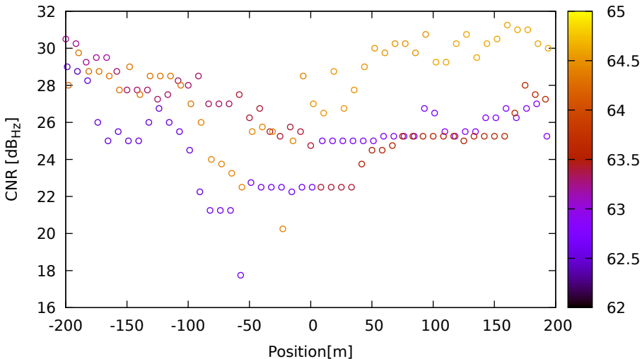
CNR vs position for G04 (L1) on Xiaomi11T - DOY 263 jam. 1
