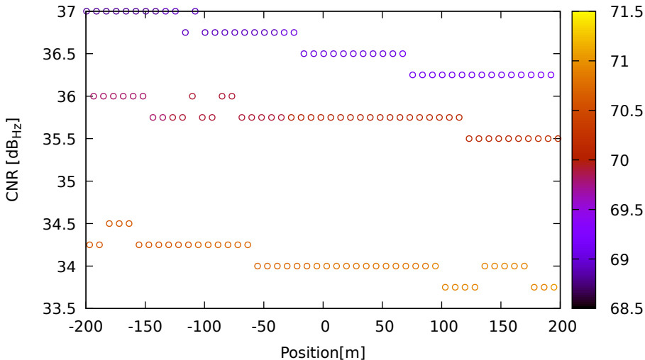
CNR vs position for G04 (L5) on Xiaomi11T - DOY 263 jam. 3
