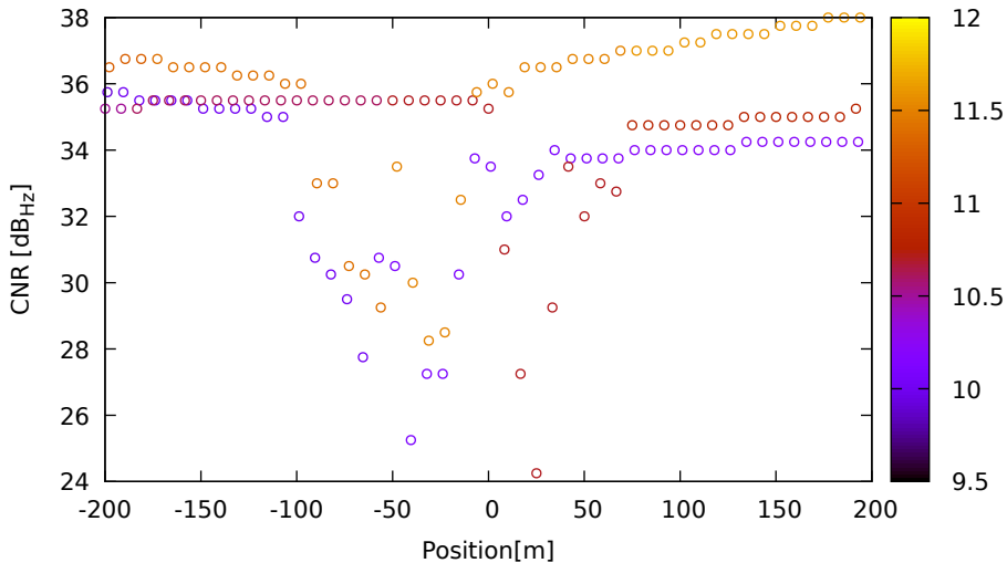
CNR vs position for G06 (L1) on Xiaomi11T - DOY 263 jam. 1
