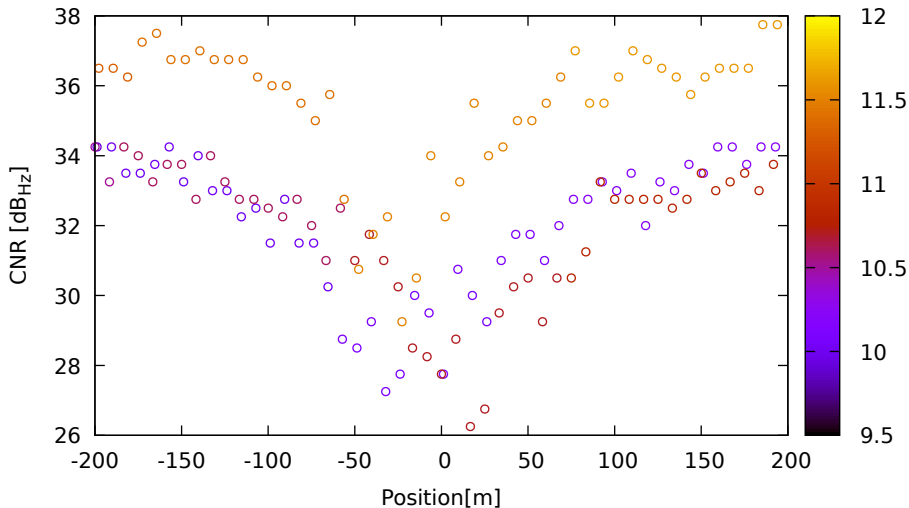
CNR vs position for G06 (L5) on Xiaomi11T - DOY 263 jam. 1
