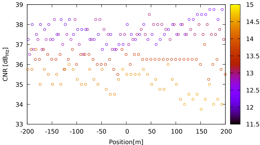
CNR vs position for G06 (L5) on Xiaomi11T - DOY 263 jam. 2
