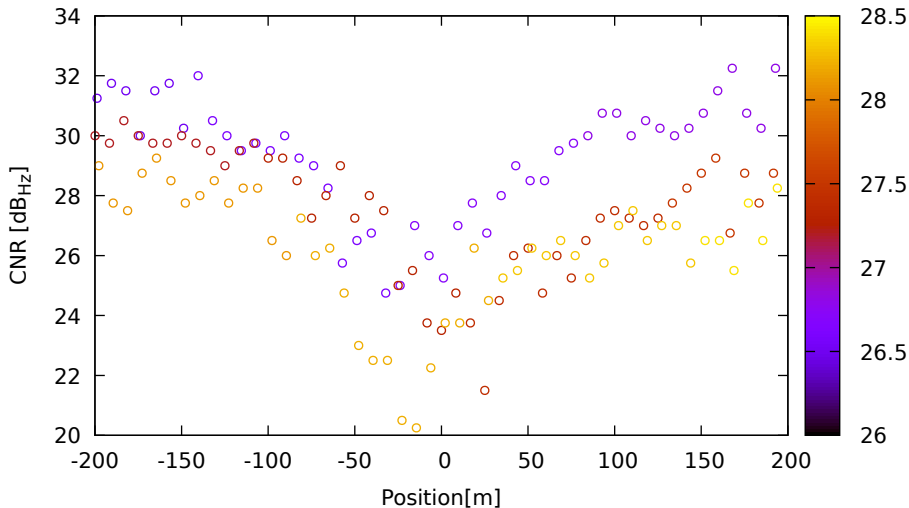
CNR vs position for G09 (L5) on Xiaomi11T - DOY 263 jam. 1
