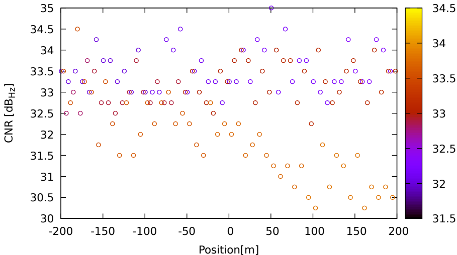
CNR vs position for G09 (L5) on Xiaomi11T - DOY 263 jam. 3
