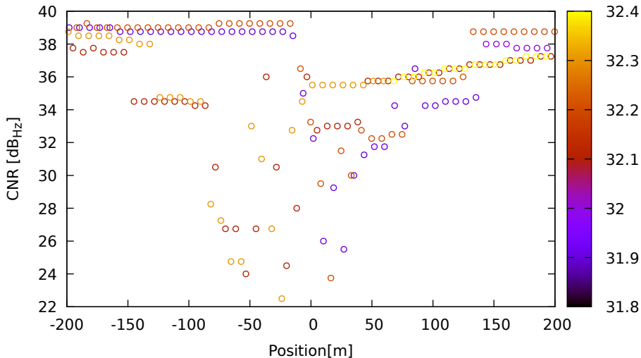
CNR vs position for G19 (L1) on Xiaomi11T - DOY 263 jam. 2
