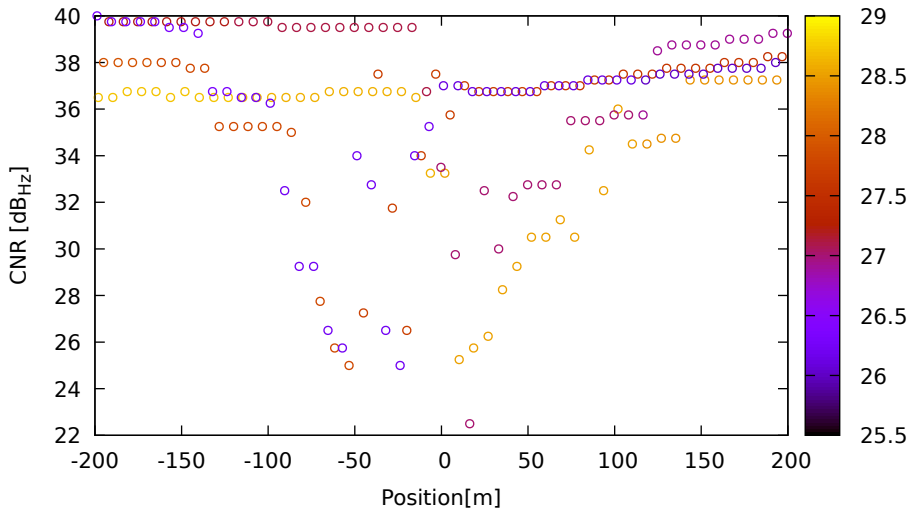
CNR vs position for G21 (L1) on Xiaomi11T - DOY 263 jam. 2
