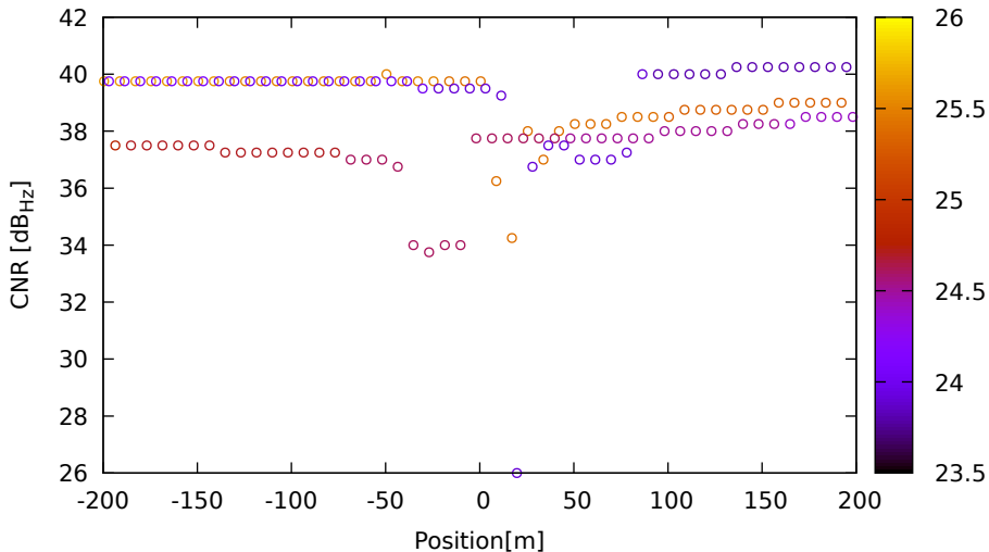
CNR vs position for G21 (L1) on Xiaomi11T - DOY 263 jam. 3
