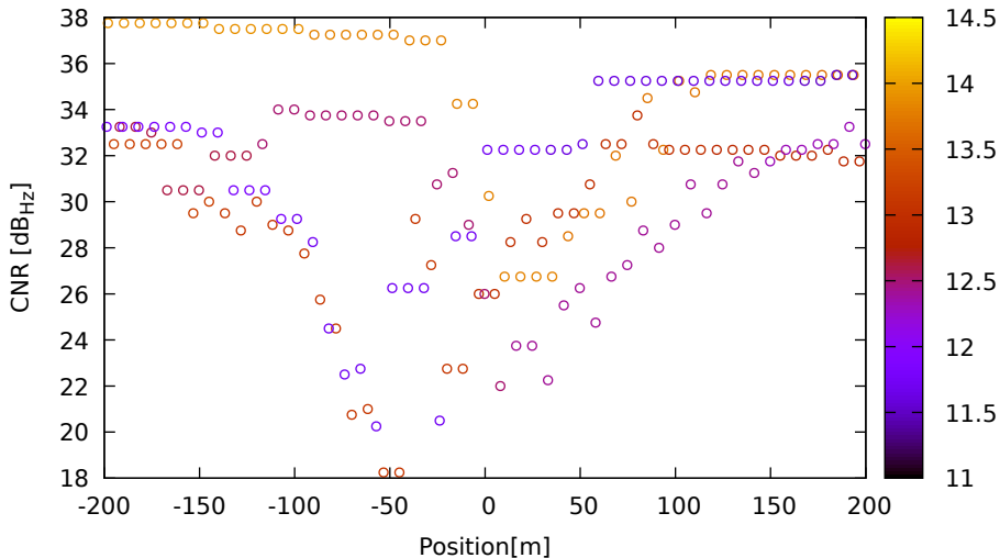
CNR vs position for G22 (L1) on Xiaomi11T - DOY 263 jam. 2
