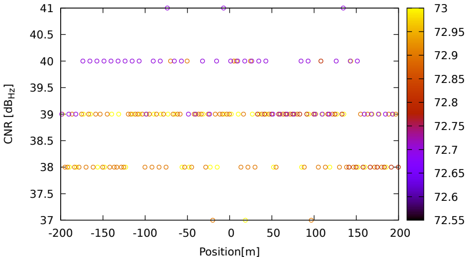
CNR vs position for R02 (G1) on Xiaomi11T - DOY 263 jam. 2
