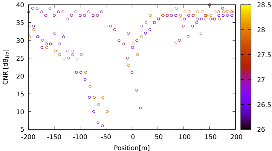
CNR vs position for R03 (G1) on Xiaomi11T - DOY 263 jam. 1
