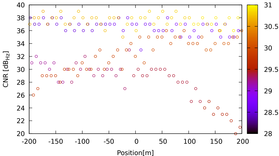
CNR vs position for R03 (G1) on Xiaomi11T - DOY 263 jam. 2
