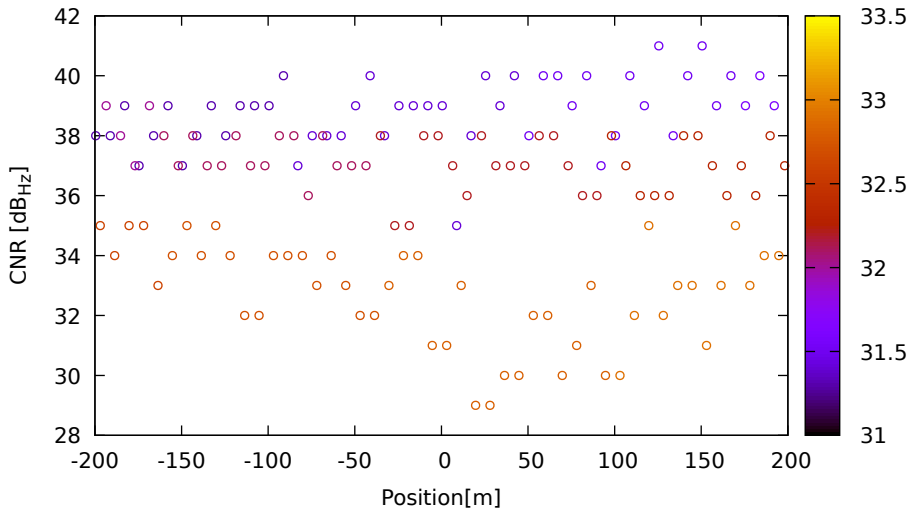
CNR vs position for R03 (G1) on Xiaomi11T - DOY 263 jam. 3
