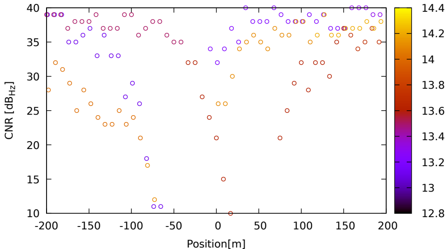
CNR vs position for R11 (G1) on Xiaomi11T - DOY 263 jam. 1
