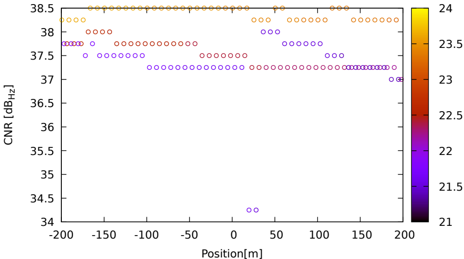
CNR vs position for R24 (G1) on Xiaomi11T - DOY 263 jam. 3
