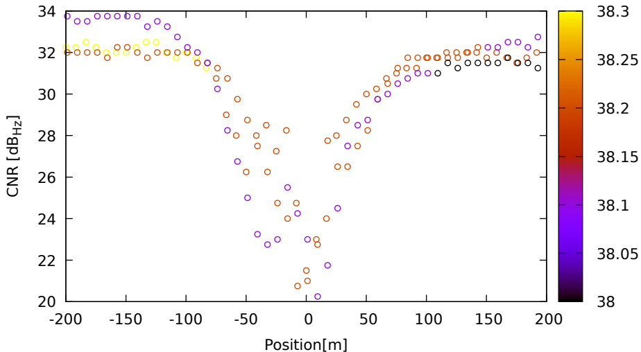
CNR vs position for C09 (B1) on XiaomiMi8 - DOY 263 jam. 1
