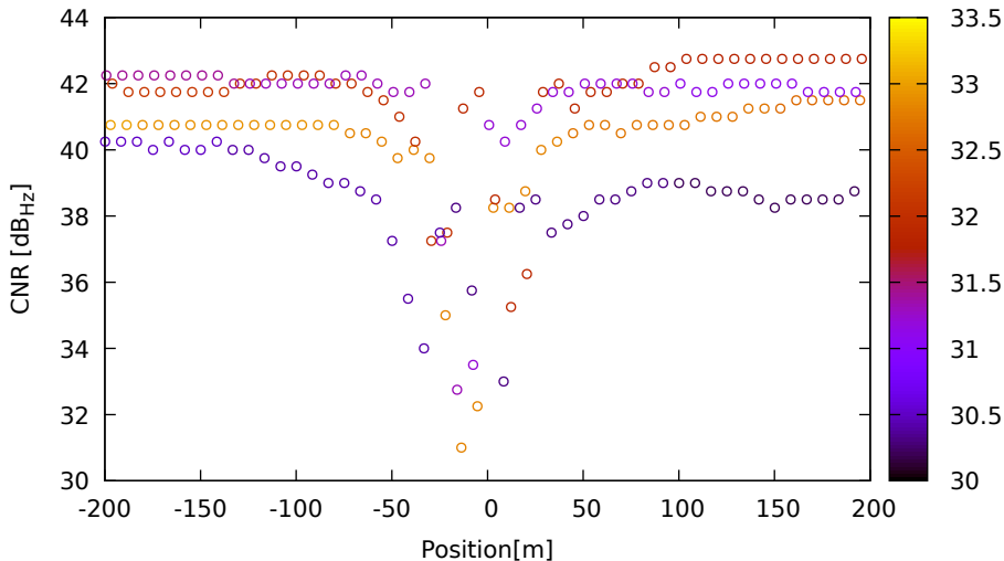
CNR vs position for C11 (B1) on XiaomiMi8 - DOY 263 jam. 2
