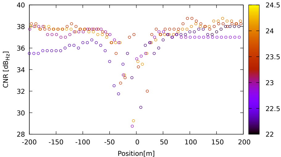
CNR vs position for C21 (B1) on XiaomiMi8 - DOY 263 jam. 2
