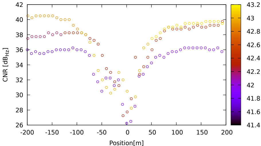
CNR vs position for C33 (B1) on XiaomiMi8 - DOY 263 jam. 1
