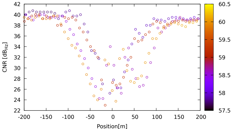
CNR vs position for E04 (E1) on XiaomiMi8 - DOY 263 jam. 2
