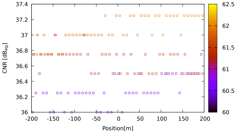
CNR vs position for E04 (E5a) on XiaomiMi8 - DOY 263 jam. 3
