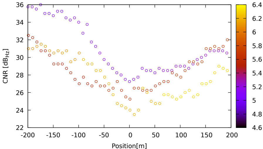
CNR vs position for E09 (E5a) on XiaomiMi8 - DOY 263 jam. 1
