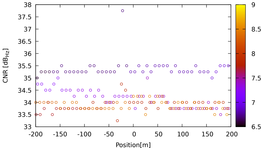
CNR vs position for E09 (E5a) on XiaomiMi8 - DOY 263 jam. 2
