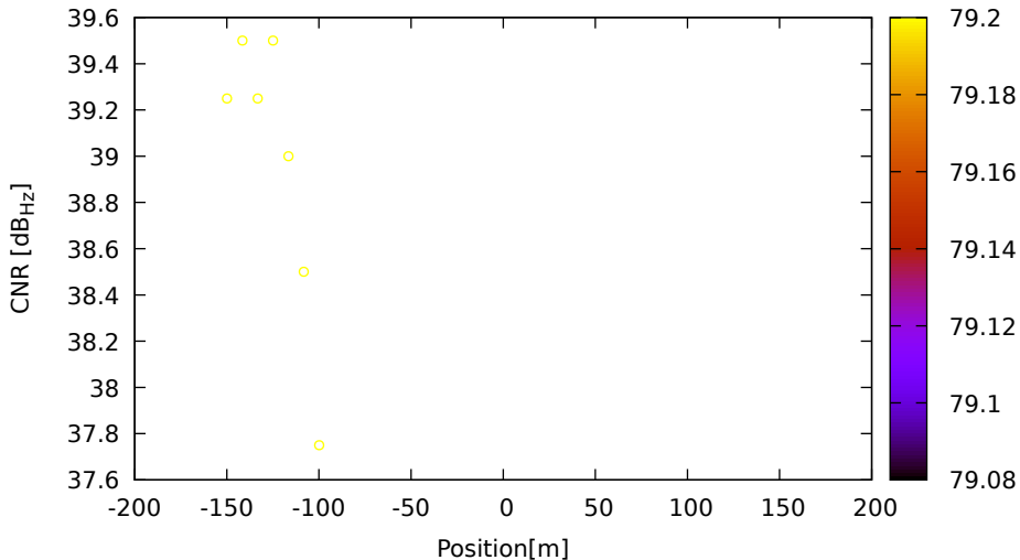
CNR vs position for E10 (E1) on XiaomiMi8 - DOY 263 jam. 1
