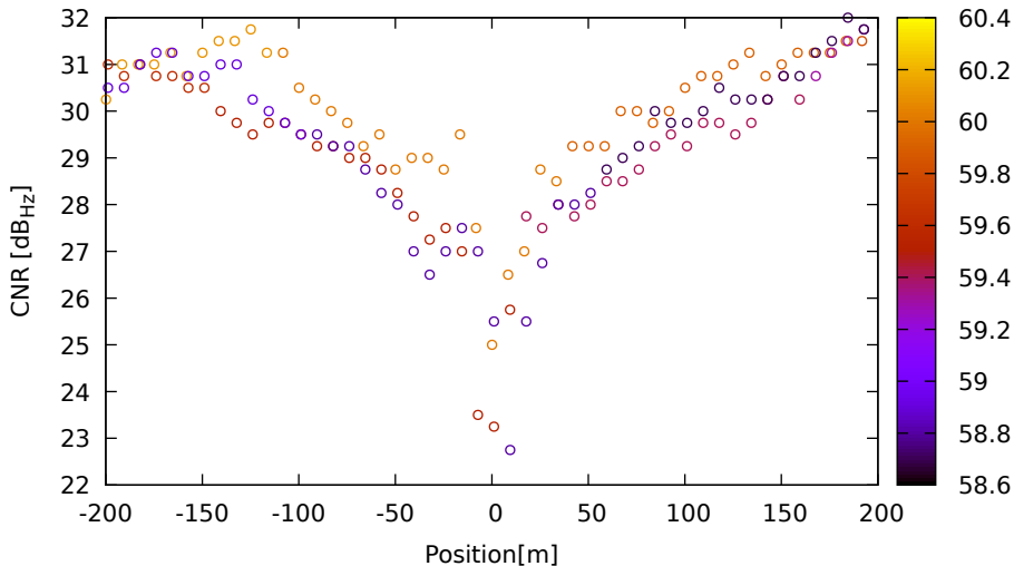
CNR vs position for E19 (E1) on XiaomiMi8 - DOY 263 jam. 1
