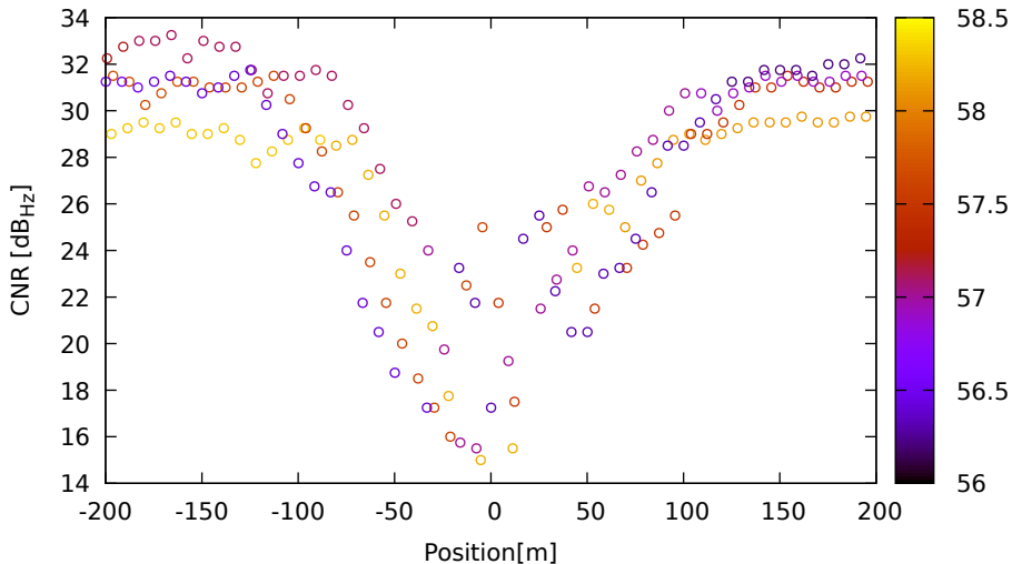
CNR vs position for E19 (E1) on XiaomiMi8 - DOY 263 jam. 2
