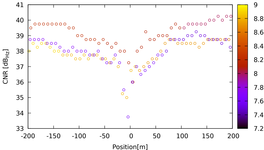
CNR vs position for E33 (E1) on XiaomiMi8 - DOY 263 jam. 3
