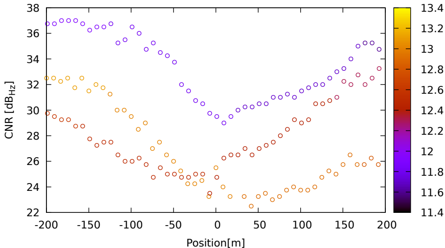
CNR vs position for E33 (E5a) on XiaomiMi8 - DOY 263 jam. 1
