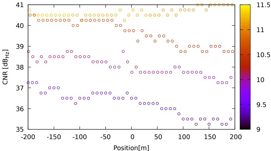
CNR vs position for E33 (E5a) on XiaomiMi8 - DOY 263 jam. 2
