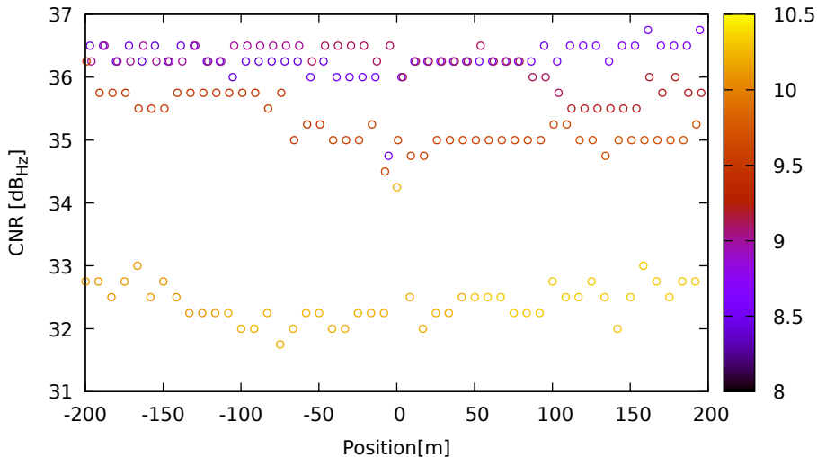
CNR vs position for E36 (E5a) on XiaomiMi8 - DOY 263 jam. 2
