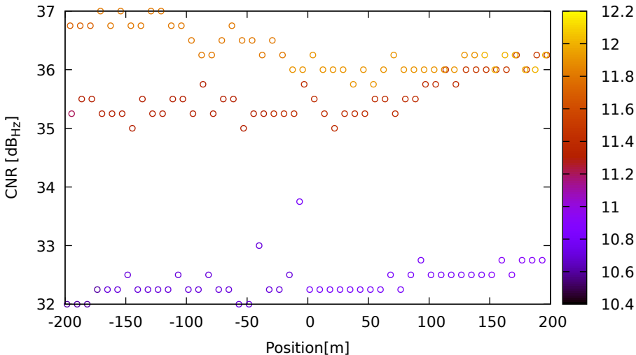
CNR vs position for E36 (E5a) on XiaomiMi8 - DOY 263 jam. 3
