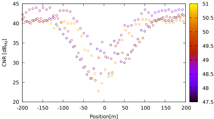
CNR vs position for G01 (L1) on XiaomiMi8 - DOY 263 jam. 2
