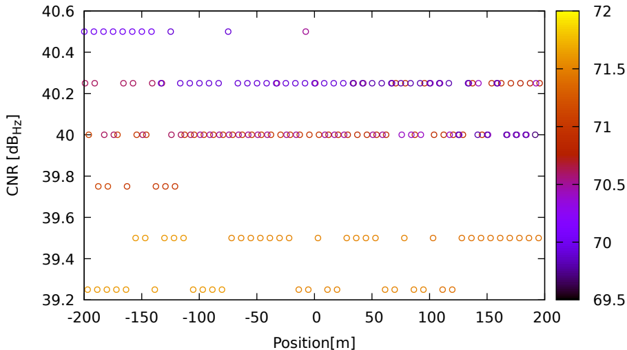
CNR vs position for G03 (L5) on XiaomiMi8 - DOY 263 jam. 2
