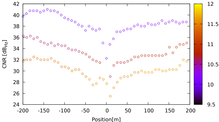
CNR vs position for G06 (L1) on XiaomiMi8 - DOY 263 jam. 1
