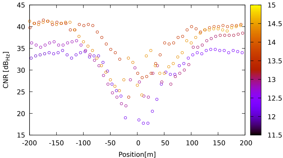
CNR vs position for G06 (L1) on XiaomiMi8 - DOY 263 jam. 2
