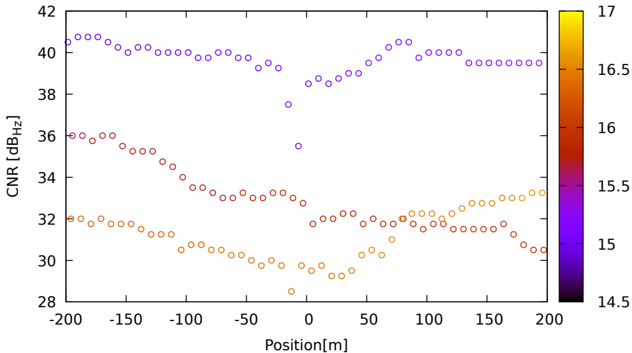
CNR vs position for G06 (L1) on XiaomiMi8 - DOY 263 jam. 3
