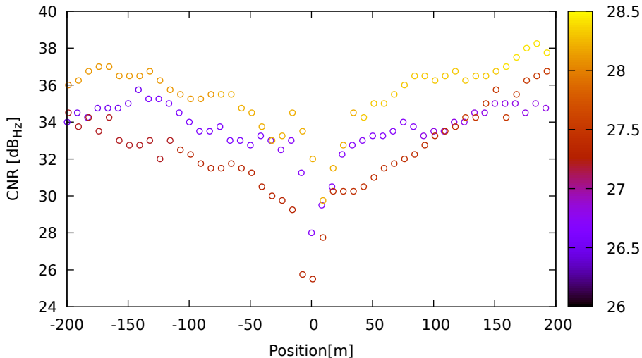
CNR vs position for G09 (L1) on XiaomiMi8 - DOY 263 jam. 1
