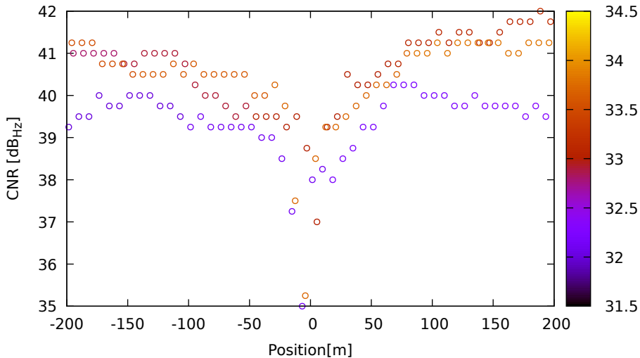
CNR vs position for G09 (L1) on XiaomiMi8 - DOY 263 jam. 3
