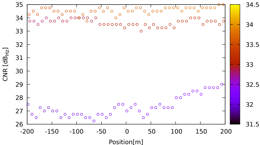
CNR vs position for G09 (L5) on XiaomiMi8 - DOY 263 jam. 3
