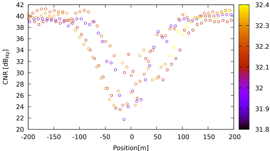
CNR vs position for G19 (L1) on XiaomiMi8 - DOY 263 jam. 2
