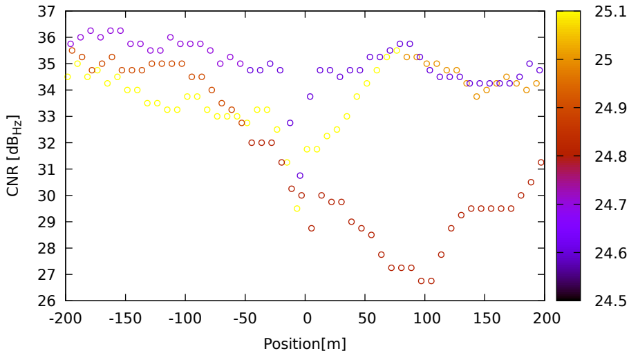
CNR vs position for G31 (L1) on XiaomiMi8 - DOY 263 jam. 3
