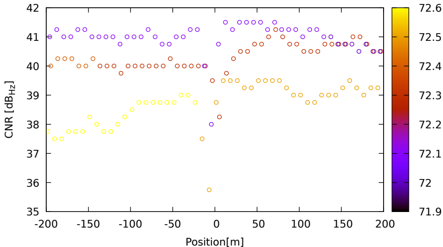
CNR vs position for R02 (G1) on XiaomiMi8 - DOY 263 jam. 3
